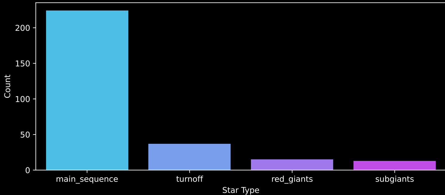
GALAH DR4 Field: [6690] Count plot of Star Type
