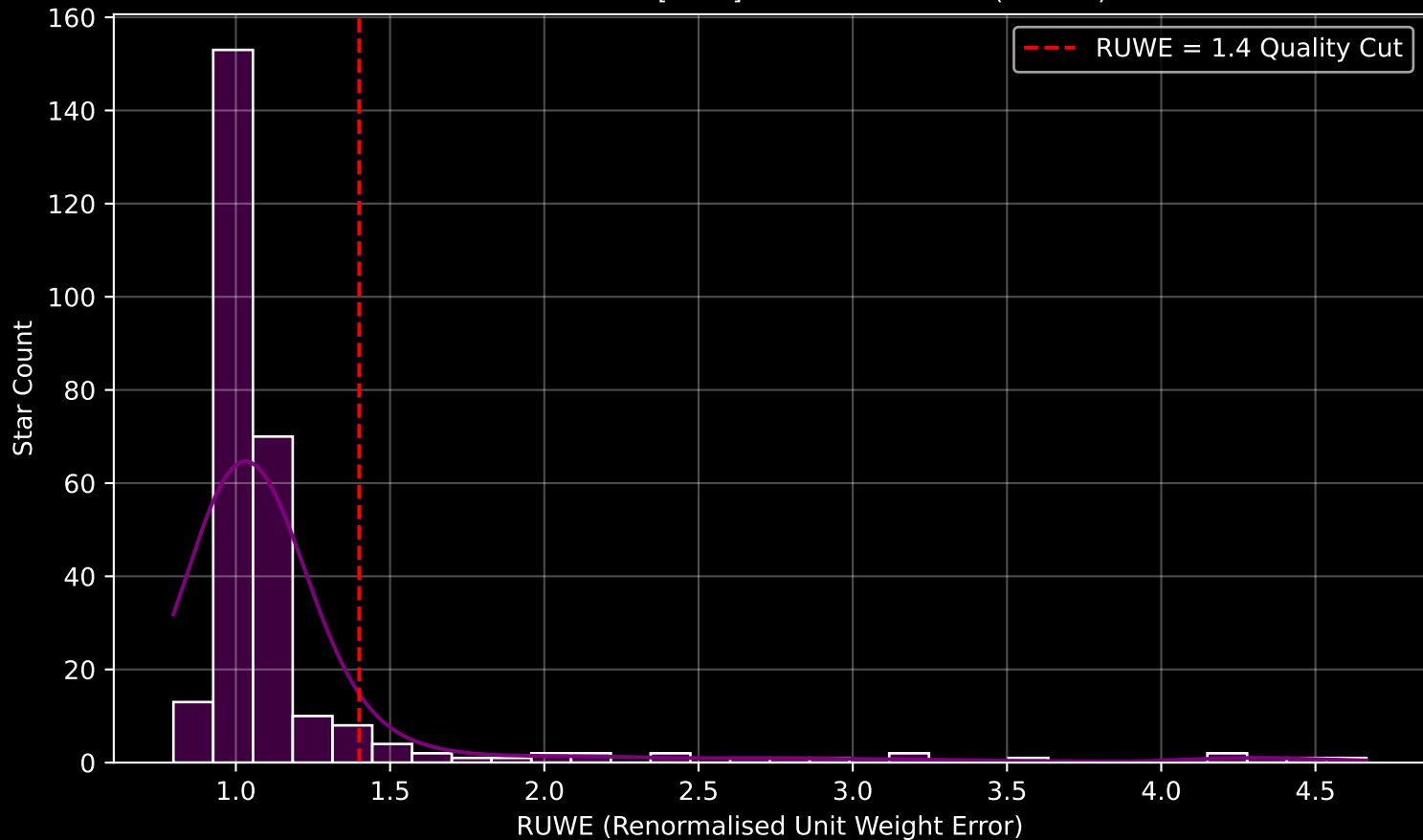
GALAH DR4 Field [6690] RUWE Distribution (n= 279)
